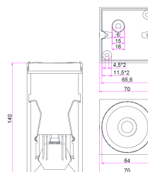
SECTION DRAWING SIDE VIEW SFIX 38D
