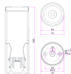
SECTION DRAWING SIDE VIEW SFIX 38D
