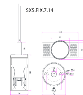
SECTION DRAWING SIDE VIEW SFIX 38D
