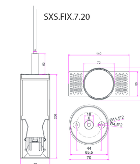
SECTION DRAWING SIDE VIEW SFIX 38D
