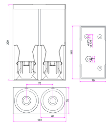
SECTION DRAWING SIDE VIEW SFIX 38D
