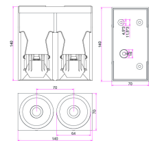
SECTION DRAWING SIDE VIEW SFIX 38D
