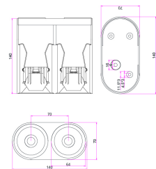
SECTION DRAWING SIDE VIEW SFIX 38D
