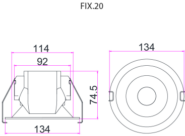
SECTION DRAWING SIDE VIEW FIX 38D CUT-OUT 92 MM
