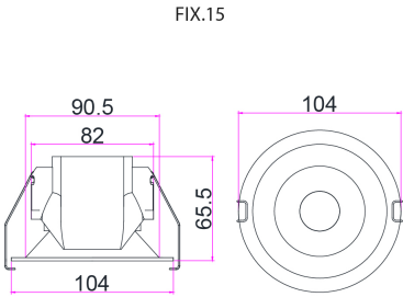
SECTION DRAWING SIDE VIEW FIX 38D CUT-OUT 90 MM
