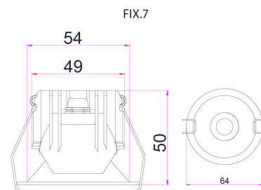
SECTION DRAWING SIDE VIEW FIX 38D CUT-OUT 55 MM
