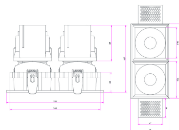
SECTION DRAWING SIDE VIEW ADJ 38D CUT-OUT 70x155 MM
