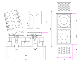
SECTION DRAWING SIDE VIEW ADJ 38D CUT-OUT 44x104 MM
