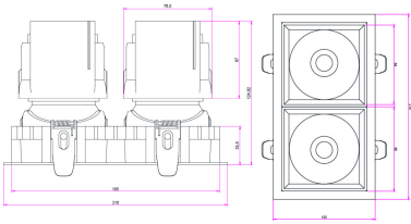
SECTION DRAWING SIDE VIEW ADJ 38D CUT-OUT 90x185 MM
