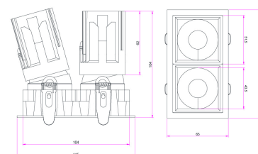
SECTION DRAWING SIDE VIEW ADJ 38D CUT-OUT 44x104 MM
