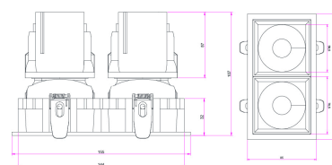
SECTION DRAWING SIDE VIEW ADJ 38D CUT-OUT 70x155 MM
