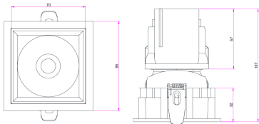
SECTION DRAWING SIDE VIEW ADJ 38D CUT-OUT 70 MM
