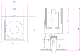
SECTION DRAWING SIDE VIEW ADJ 38D CUT-OUT 44 MM
