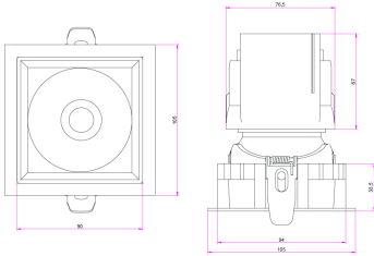
SECTION DRAWING SIDE VIEW ADJ 38D CUT-OUT 90 MM
