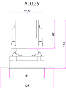
SECTION DRAWING SIDE VIEW ADJ 38D CUT-OUT 84 MM
