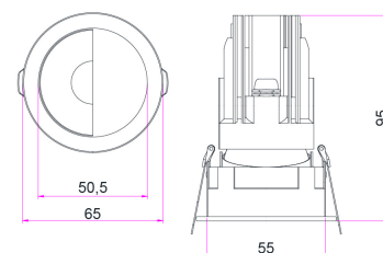
SECTION DRAWING SIDE VIEW ADJ 38D CUT-OUT 50 MM
