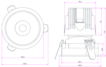
SECTION DRAWING SIDE VIEW ADJ 38D CUT-OUT 98 MM
