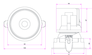
SECTION DRAWING SIDE VIEW ADJ 38D CUT-OUT 73 MM
